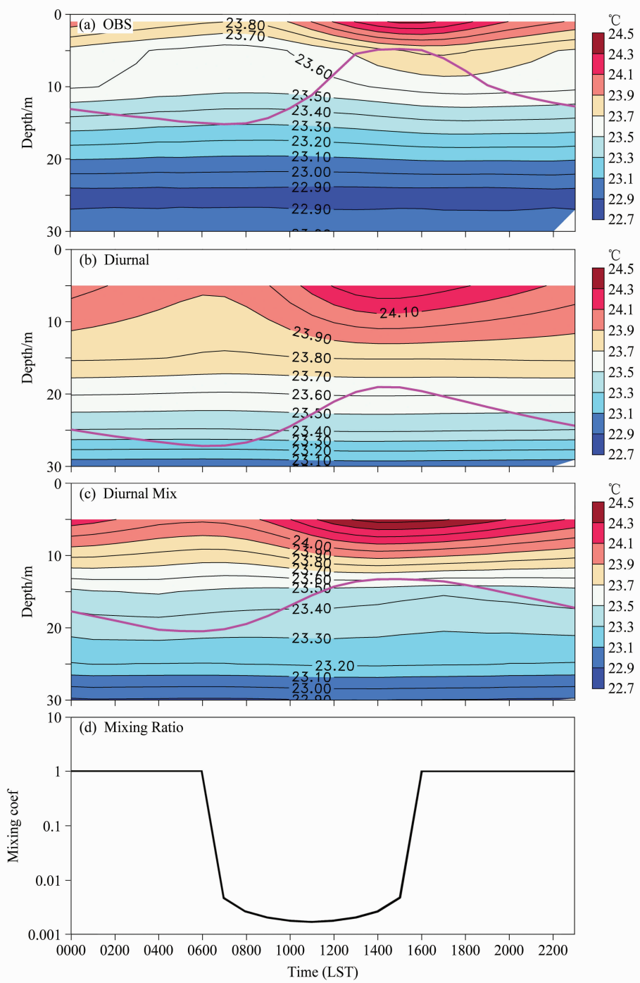
图4 赤道东太平洋冷舌区不同深度上气候态温度的日变化：(a) 位于(0°N, 110°W)的观测资料(来自TAO/TRITON, NOAA/PMEM)；(b) Diurnal 和 (c) DiurnalMix [取(2°S~2°N, 120°W~110°W)平均]。(d) 减小混合系数后第1层混合系数数量值变化。紫红色线为混合层深度(定义为与SST之差为0.5℃所在深度) Fig. 4 The climatological diurnal variation of depth - temperature in the equatorial eastern Pacific cold tongue from (a) TAO/TRITON, NOAA/PMEL observational data located at (0°N, 110°W), (b) Diurnal and (c) DiurnalMix expts [averaged over (2°S - 2°N, 120°W - 110°W)]. (d) The change of mixing coefficient magnitude in the first layer after reducing the mixing coefficient. The purple line is for mixed layer depth (defined by the depth at which the difference between SST and temperature is about 0.5℃)
