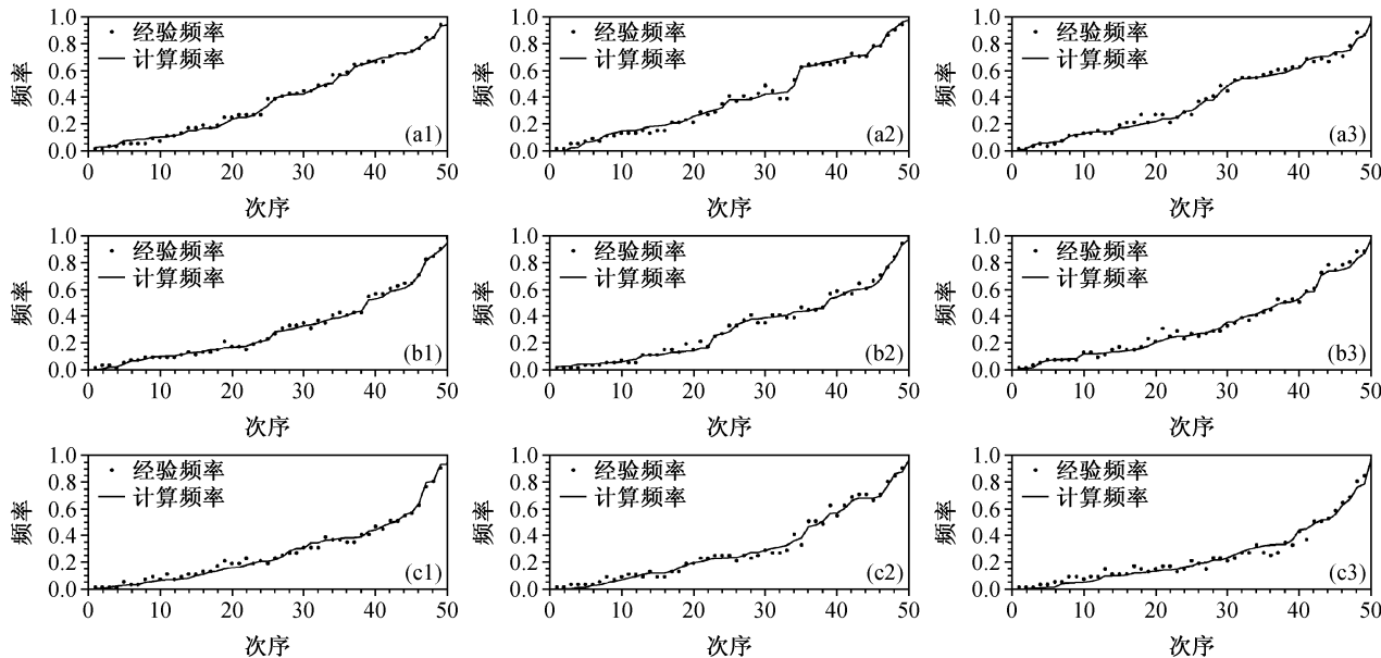
图2 水源区与各受水区在汛期（左列）、非汛期（中列）和全年（右列）的计算频率和经验频率的拟合：（a1、a2、a3）汉唐遭遇；（b1、b2、b3）汉黄遭遇；（c1、c2、c3）汉海遭遇 Fig.2 The calculated and empirical frequencies between water source area and water receiving areas for the flood season (left panel), non-flood season (middle panel), and the whole year (right panel): (a1, a2, a3) Han - Tang encounter; (b1, b2, b3) Han - Huang encounter; (c1, c2, c3) Han - Hai encounter
