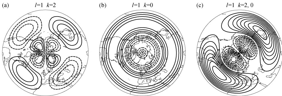
图 9 经向波数和纬向波数满足 (a) l=1, k=2 和 (b) l=1, k=0 的高度场异常空间分布以及 (c) 两种高度场异常的叠加 (单位: gpm)。等值线间隔: 4 gpm; 实线: 正异常; 虚线: 负异常; 图中省略了零线 Fig. 9 The geopotential height anomalies (gpm) when (a) l=1, k=2 and (b) l=1, k=0 ; (c) the sum of the geopotential height anomalies in (a) and (b). Isolines are drawn every 4 gpm, solid and dashed lines indicate the positive and negative anomalies respectively, and the zero lines are omitted
